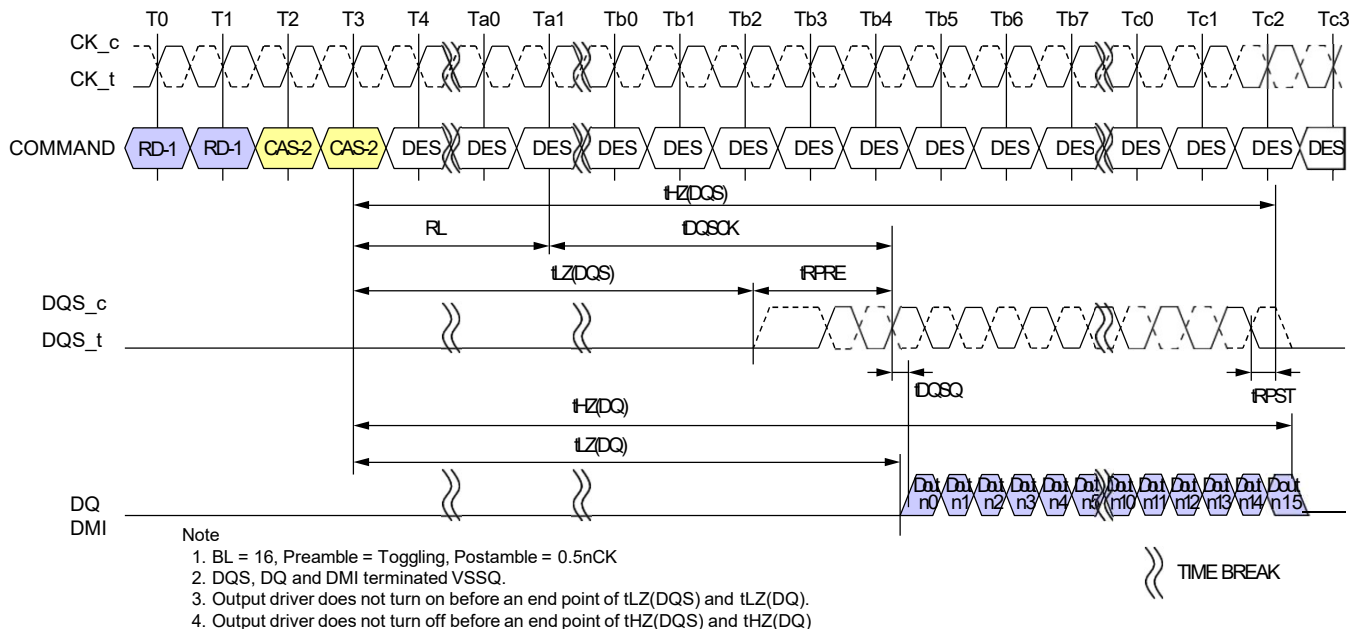
Figure 12 - Read Timing
