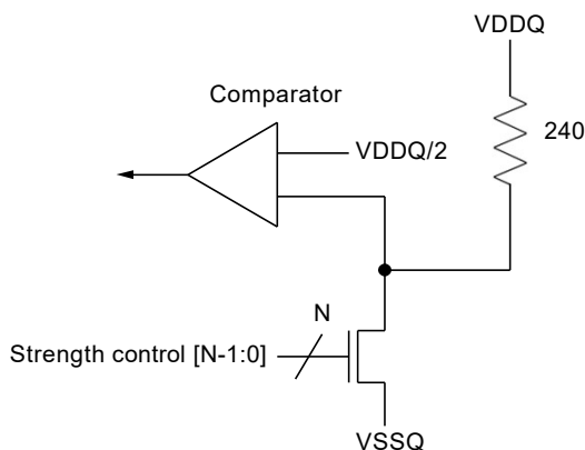
Figure 181 - Pull-down calibration
