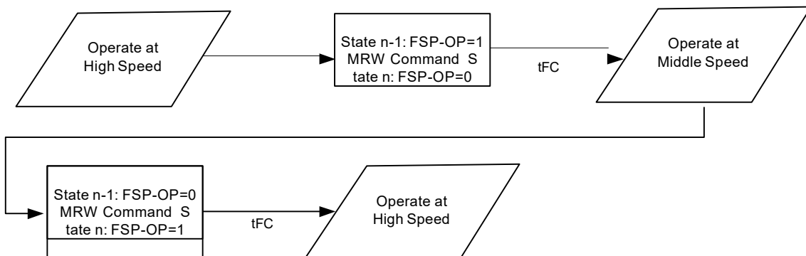
Figure 105 - Switching between two trained Frequency Set Points
