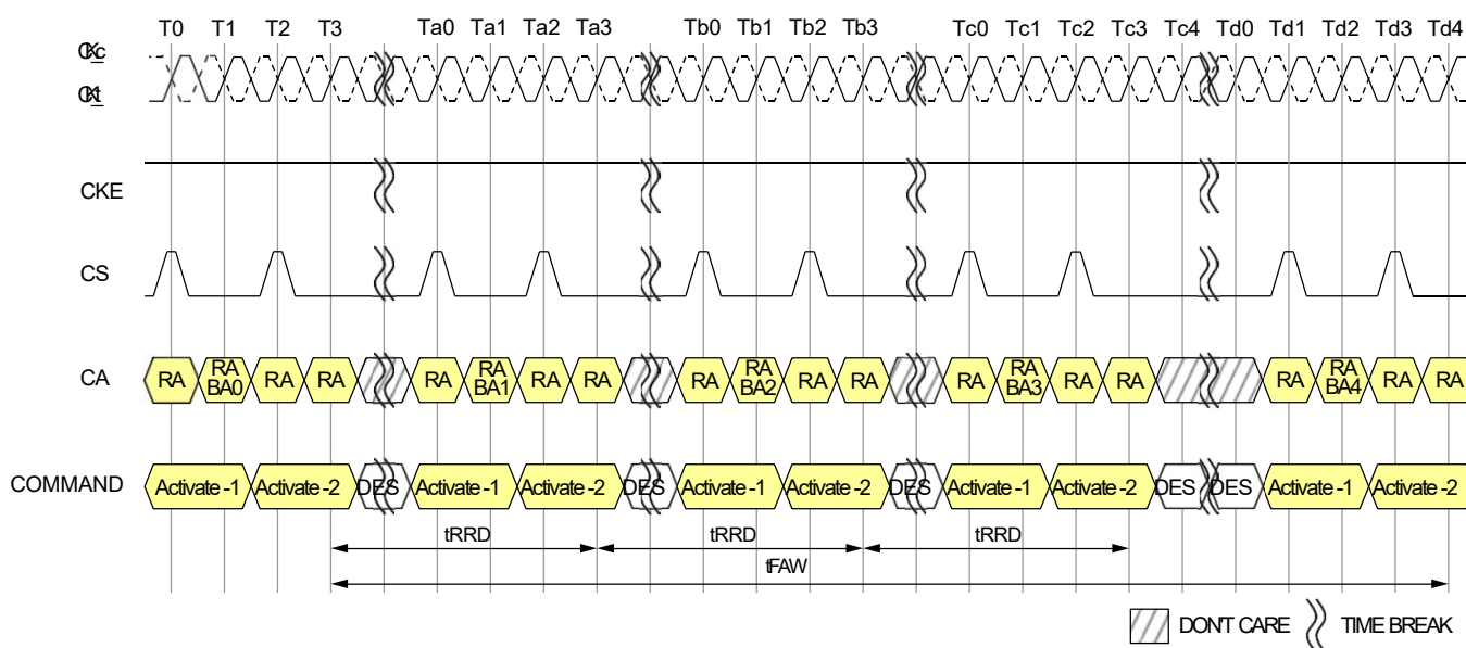
Figure 6 - tFAW Timing
