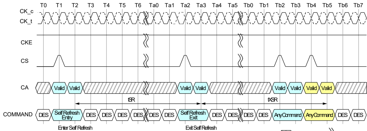
Figure 72 - Self Refresh Entry/Exit Timing
