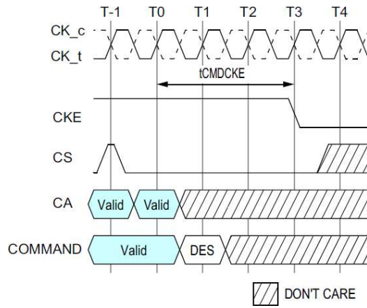
Figure 160 - t_{CMDCKE} Timing
