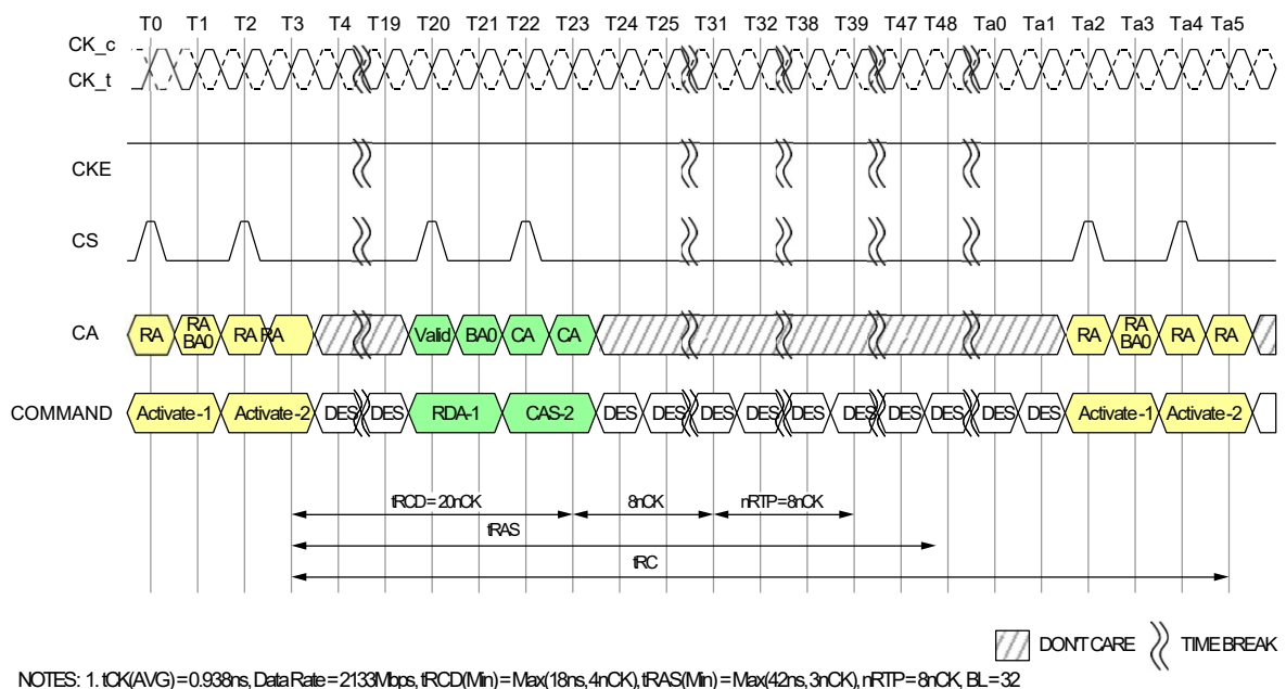
Figure 60 - Command Input Timing with RAS lock
