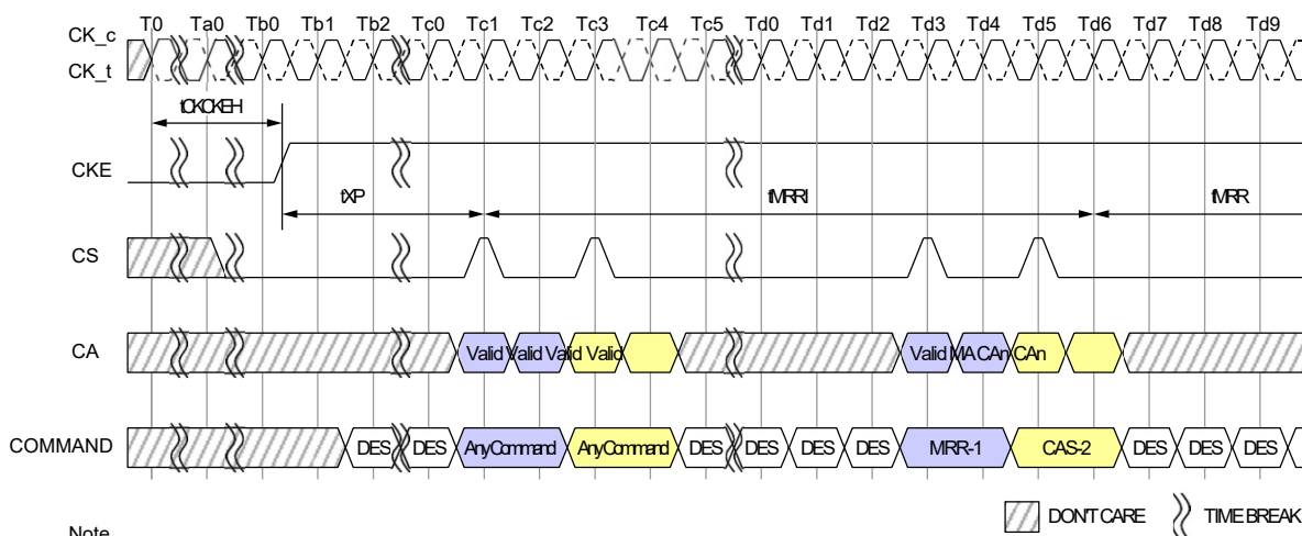
Figure 81 - MRR Following Power-Down
