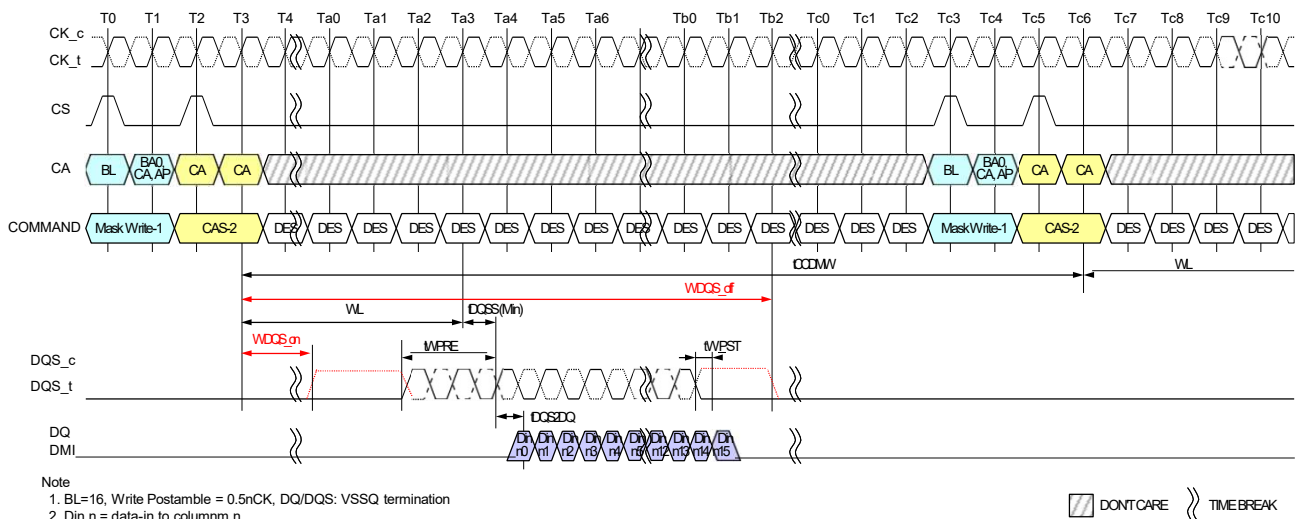
Figure 53 - Masked Write Command - Same Bank
