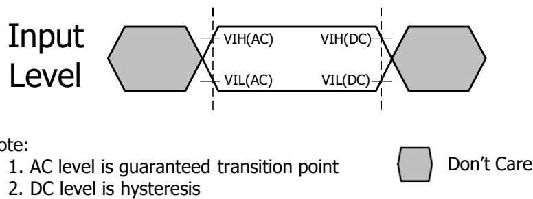
Figure 163 - Input AC timing definition for CKE
