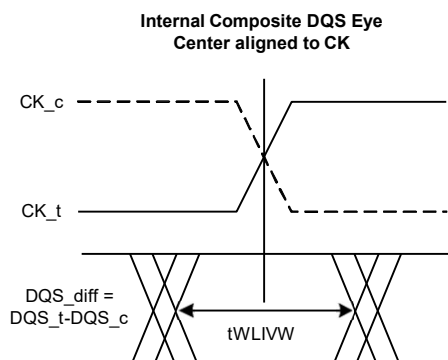
Figure 110 - DQS_t/DQS_c and CK_t/CK_c at DRAM Latch
