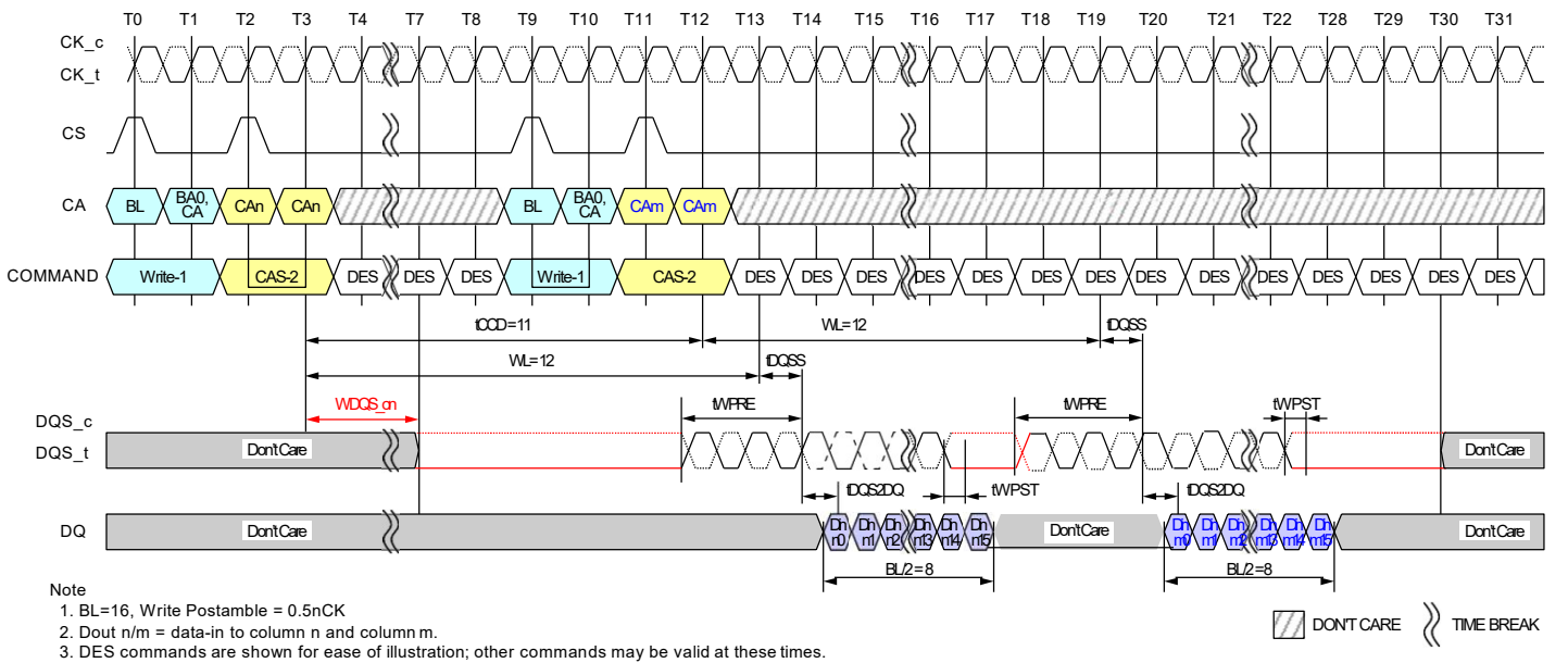
Figure 50 - Consecutive Writes Operation: t_{CCD} = \text{Min} + 3, 0.5n\text{CK} Postamble
