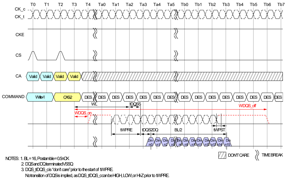
Figure 20 - DQS Write Preamble and Postamble; 0.5nCK Postamble
